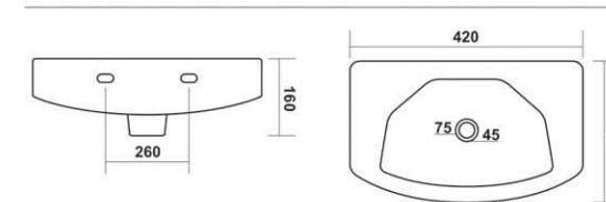
3008 - REX L 420, W 290, H 160mm
