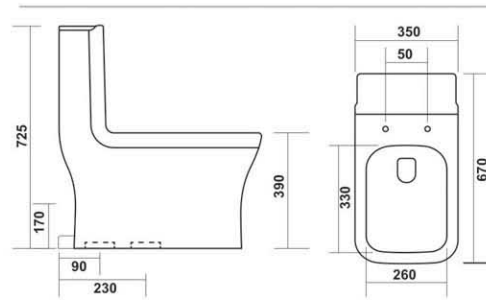
1001 - FLAT (Wash Down) L 670, W 350, H 725mm S Trap - 225mm, 100mm. P Trap - 180mm
