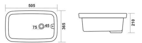
201 - LAB SINK L 505, W 365, H 210mm
