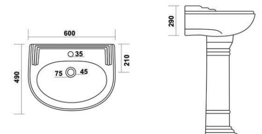
SERENA SET - WB 8006 - PED 9005 L 600, W 490, H 950mm
