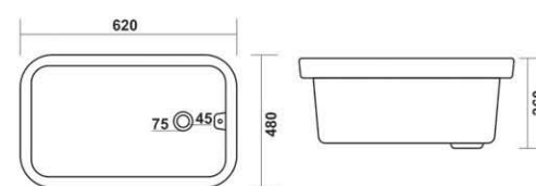
202 - LAB SINK L 620, W 480, H 260mm
