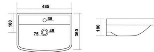
3015 - DOVEL L 485, W 360, H 180mm
