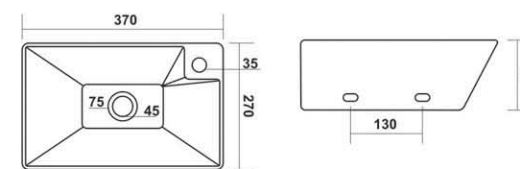
3016 - RUBI L 370, W 270, H 130mm
