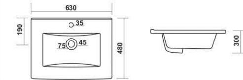
101 - AQUA TOP COUNTER L 630, W 480, H 300mm
