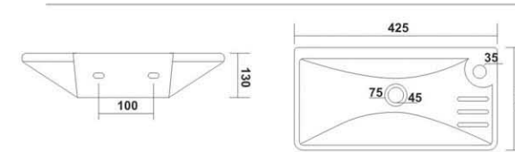
3006 - YETI L 425, W 250, H 130mm
