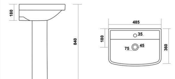
DOVEL SET - WB 3015 - PED 9014 L 485, W 360, H 840mm
