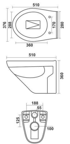
2013 - MASSIVE L 510, W 376, H 360mm
