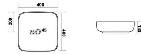
7019 - CLASSIC L 400, W 400, H 130mm
