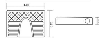
5013 - SQUATTING L 470, W 370, H 100mm
