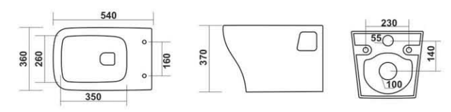
2005 - MARVEL L 540, W 360, H 370mm
