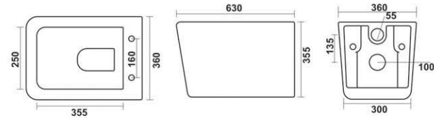
2009 - MINTO L 630, W 360, H 355mm
