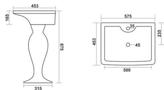
PENGVIN SET - WB 8013 - PED 9006 L 575, W 453, H 875mm
