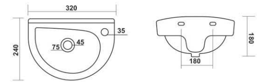
3012 - SHARP L 320, W 240, H 180mm
