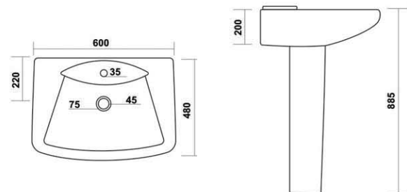
SIMON SET - WB 8009 - PED 9007 L 600, W 480, H 885mm
