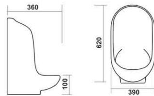
5010 - LARGE URINAL L 390, W 360, H 620mm
