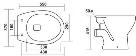
6002 - EWC 'P' L 550, W 370, H 415mm
