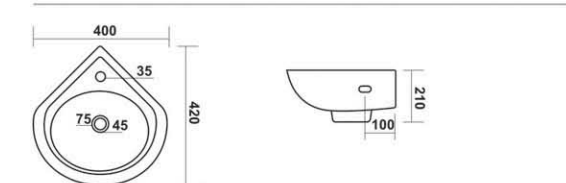
3007 - CORNER L 420, W 400, H 210mm
