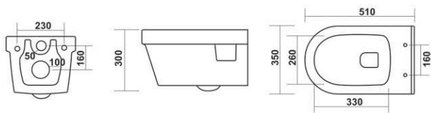
2002 - MEGA L 510, W 350, H 300mm
