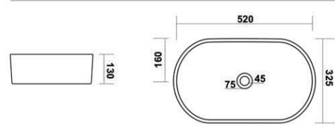
7002 - CAPSULE L 520, W 325, H 130mm
